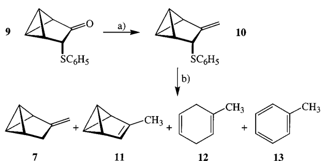
Scheme 2. a) \text{Ph}_3\text{PMe}^+\text{Br}^- , \text{KOtBu} , \text{Et}_2\text{O} , 20 °C; b) \text{Na} , liquid \text{NH}_3 , \text{EtOH} , \text{Et}_2\text{O} , -70 to -60 °C
